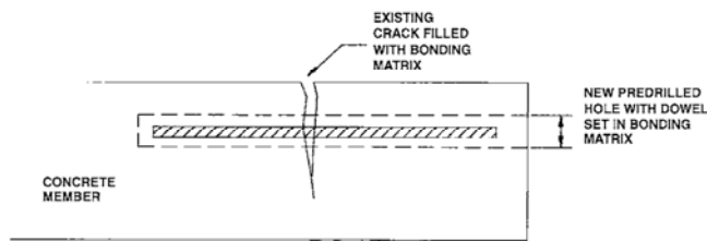
Fig. 5.1—Interior reinforcement provides increased tensile resistance to an existing crack when bonded in a predrilled hole or groove cut perpendicular to the crack.
