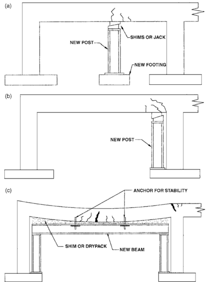
Fig. 5.8—Supplemental members.
