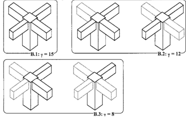
Fig. 4.5— \gamma -values for Type 2 connections.
