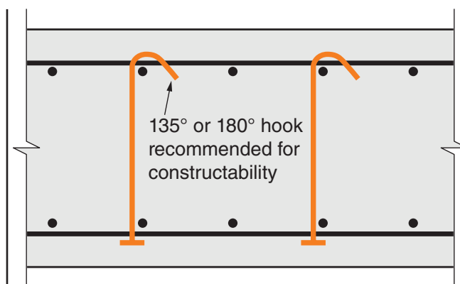
(a) Headed stirrups in a mat foundation
