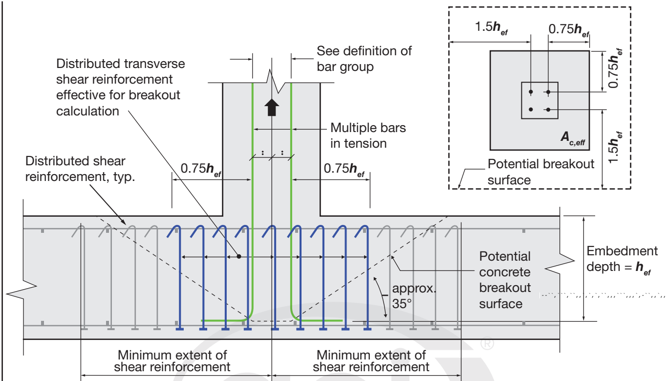
Fig. R25.4.11.5a—Use of shear reinforcement to increase the breakout strength of a group of column bars in tension
