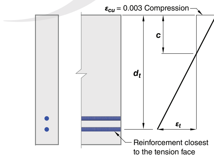
Fig. R21.2.2a—Strain distribution and net tensile strain in a nonprestressed member.
