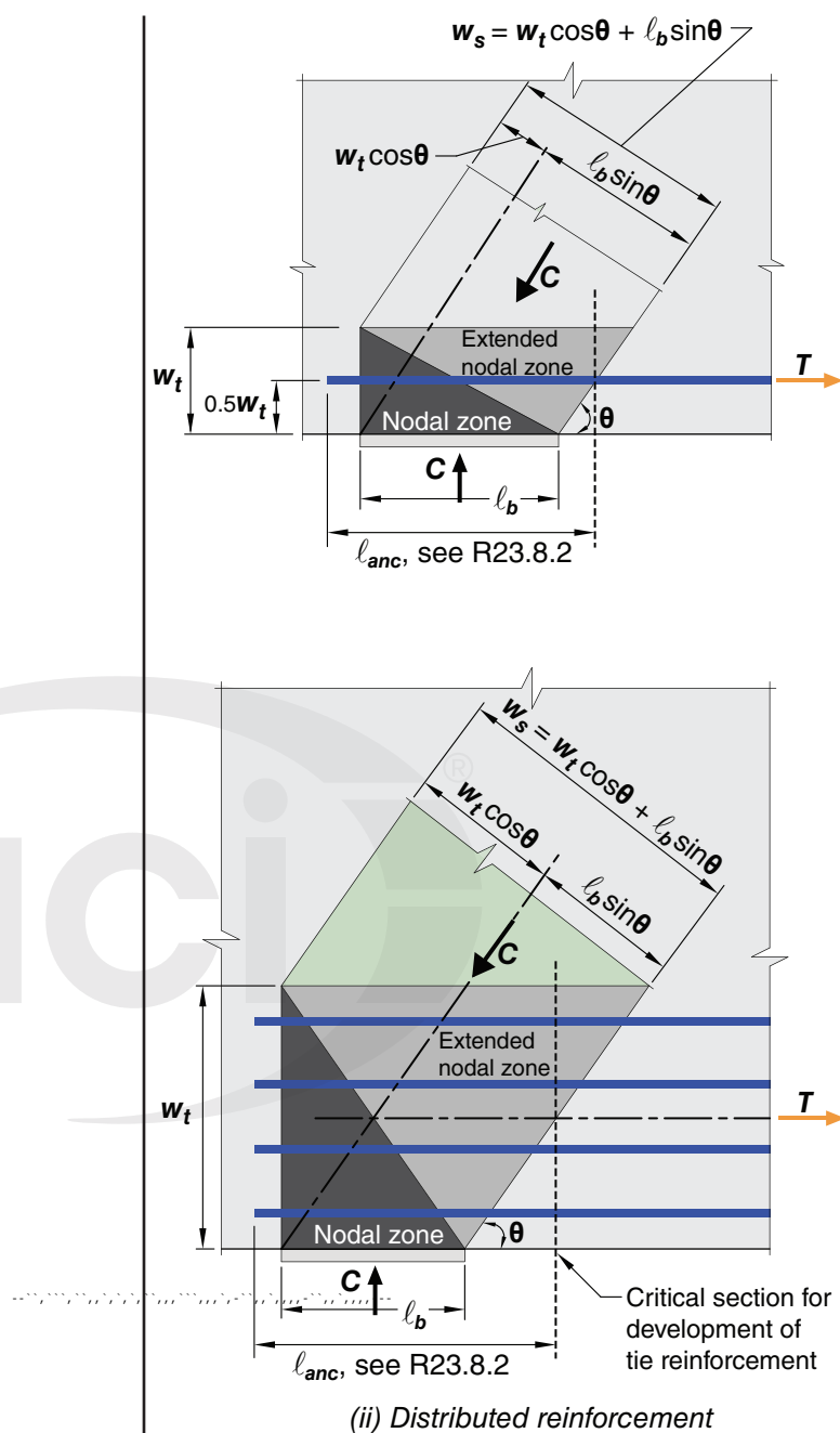
Fig. R23.2.6b—Extended nodal zone showing the effect of the distribution of the force.
