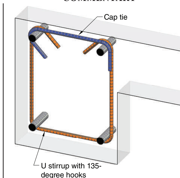
Fig. R25.7.1.6.1—Example of a two-piece stirrup that complies with the requirements of 25.7.1.6.1.
