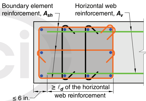
Fig. R18.10.6.4d Development of wall horizontal reinforcement in confined boundary element.
