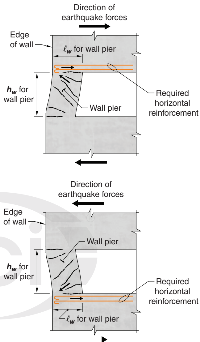
Fig. R18.10.8—Required horizontal reinforcement in wall segments above and below wall piers at the edge of a wall.
