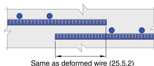
Fig. R25.5.3.1—Lap splices of welded deformed wire reinforcement.
