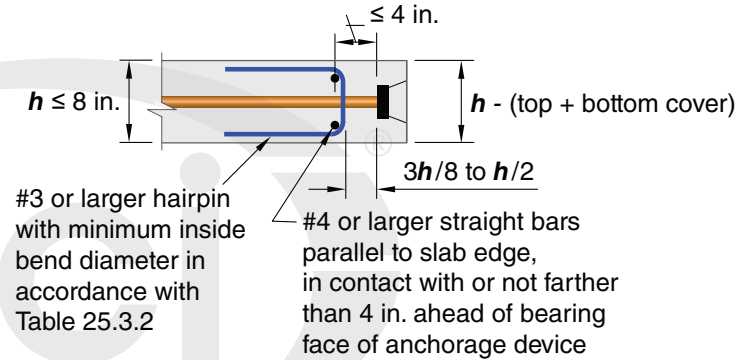
(c) Section A-A for slabs with h \leq 8 in.
