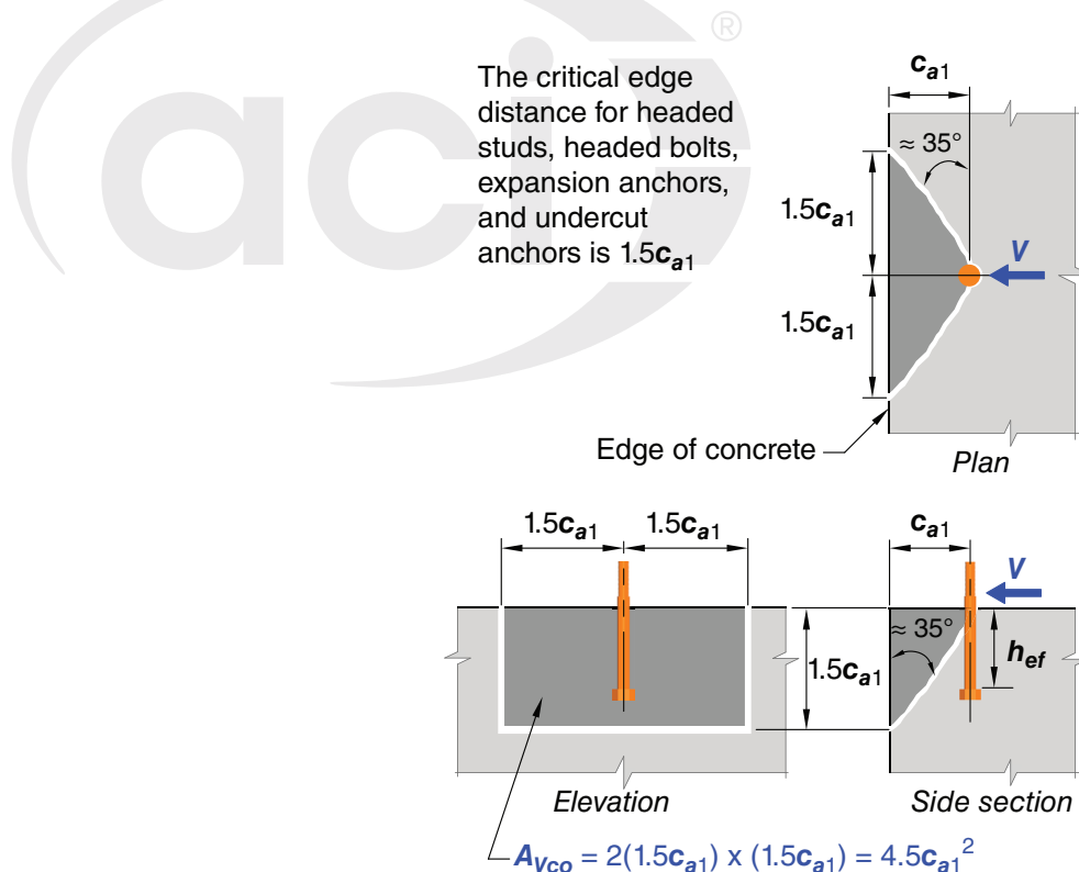
Fig. R17.7.2.1a—Calculation of A_{Vco} .
