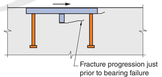
Fig. R17.11.1.1a—Examples of attachments with shear lugs.
