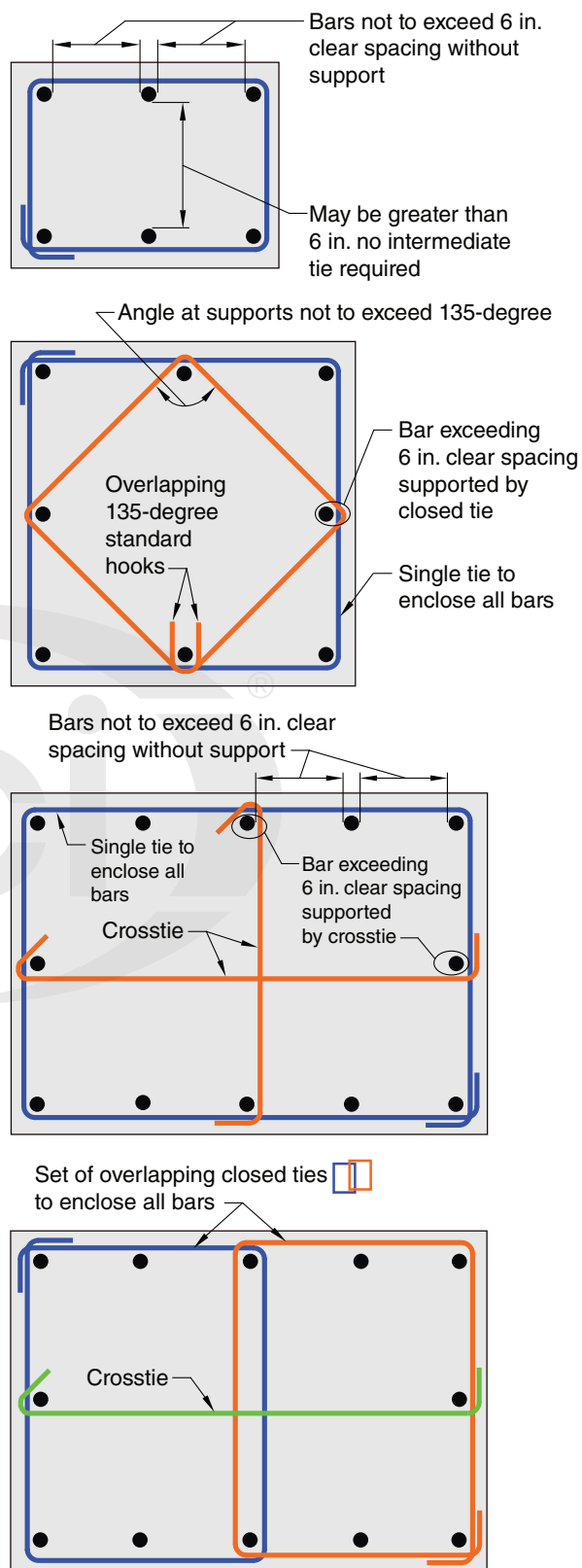
Fig. R25.7.2.3a—Illustrations to clarify measurements between laterally supported column bars and rectilinear tie anchorage.
