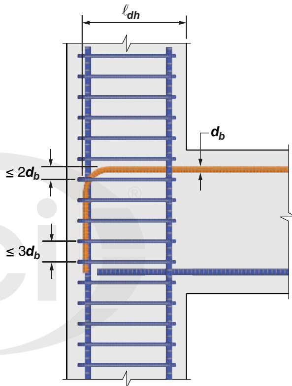
Fig. R25.4.3.2a—Ties or stirrups placed parallel to the bar being developed, spaced along the length of the tail extension of the hook plus bend.
