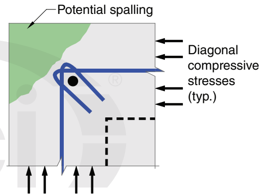
(b) Detail at corner
