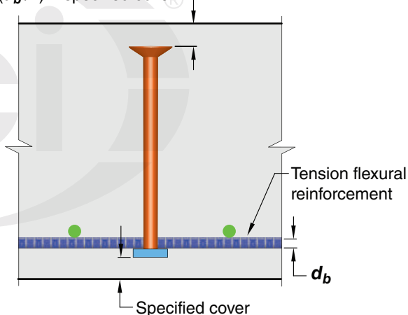
(b) Footing with only bottom bars
