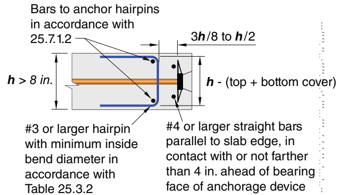
(b) Sectional A-A for slabs with h > 8 in.
