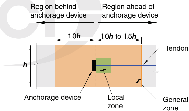
Section through slab at anchorage
