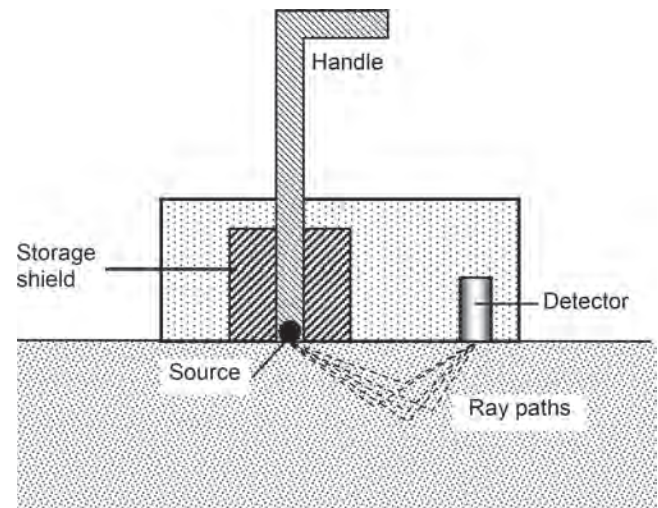
Fig. 3.4.3.2—Schematic of backscatter nuclear density gauge.
