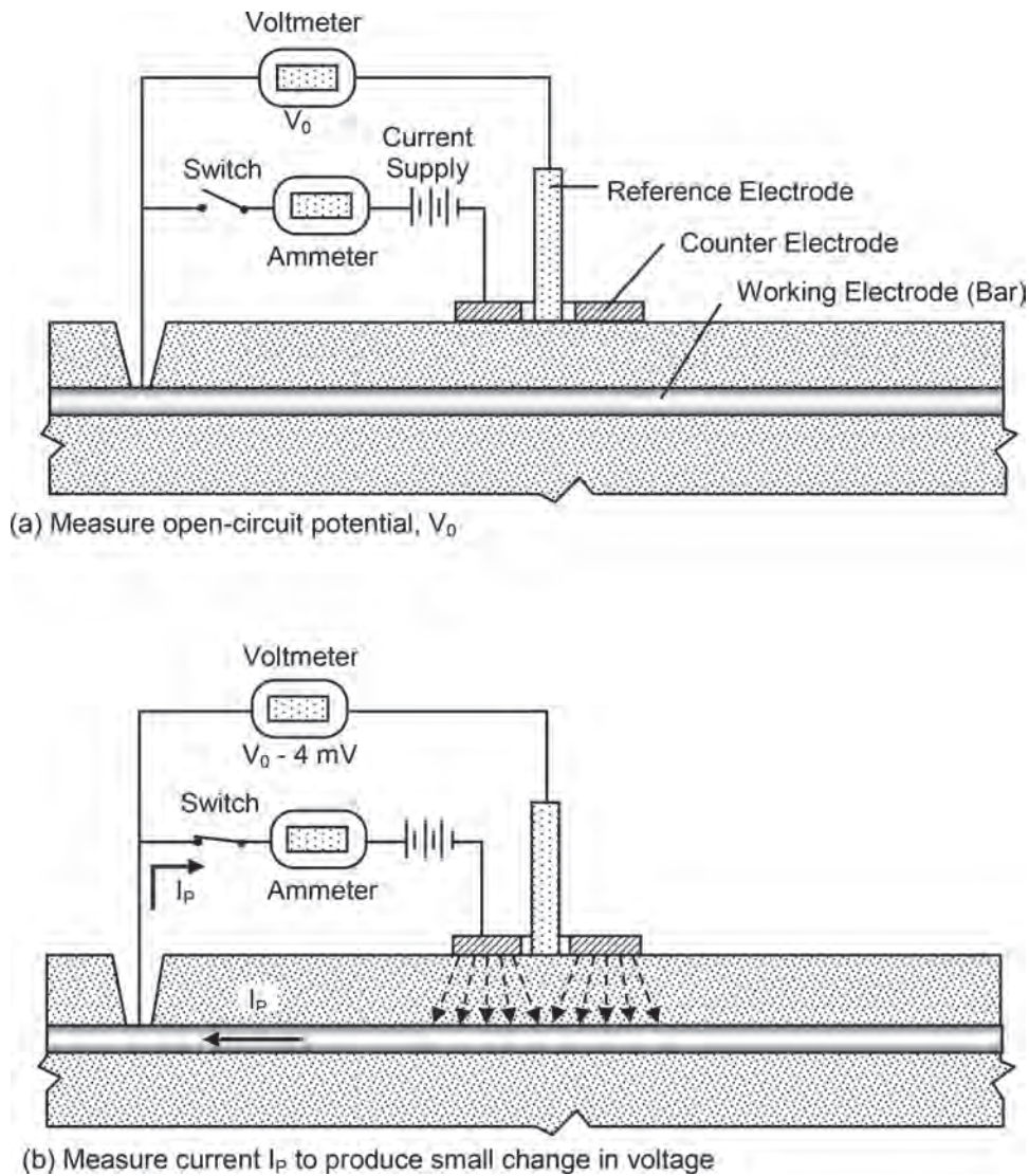
Fig. 3.5.4.2a—Three-electrode, linear-polarization method to measure corrosion current: (a) measurement of open-circuit potential; and (b) measurement of current to produce small change in potential of working electrode (bar).
