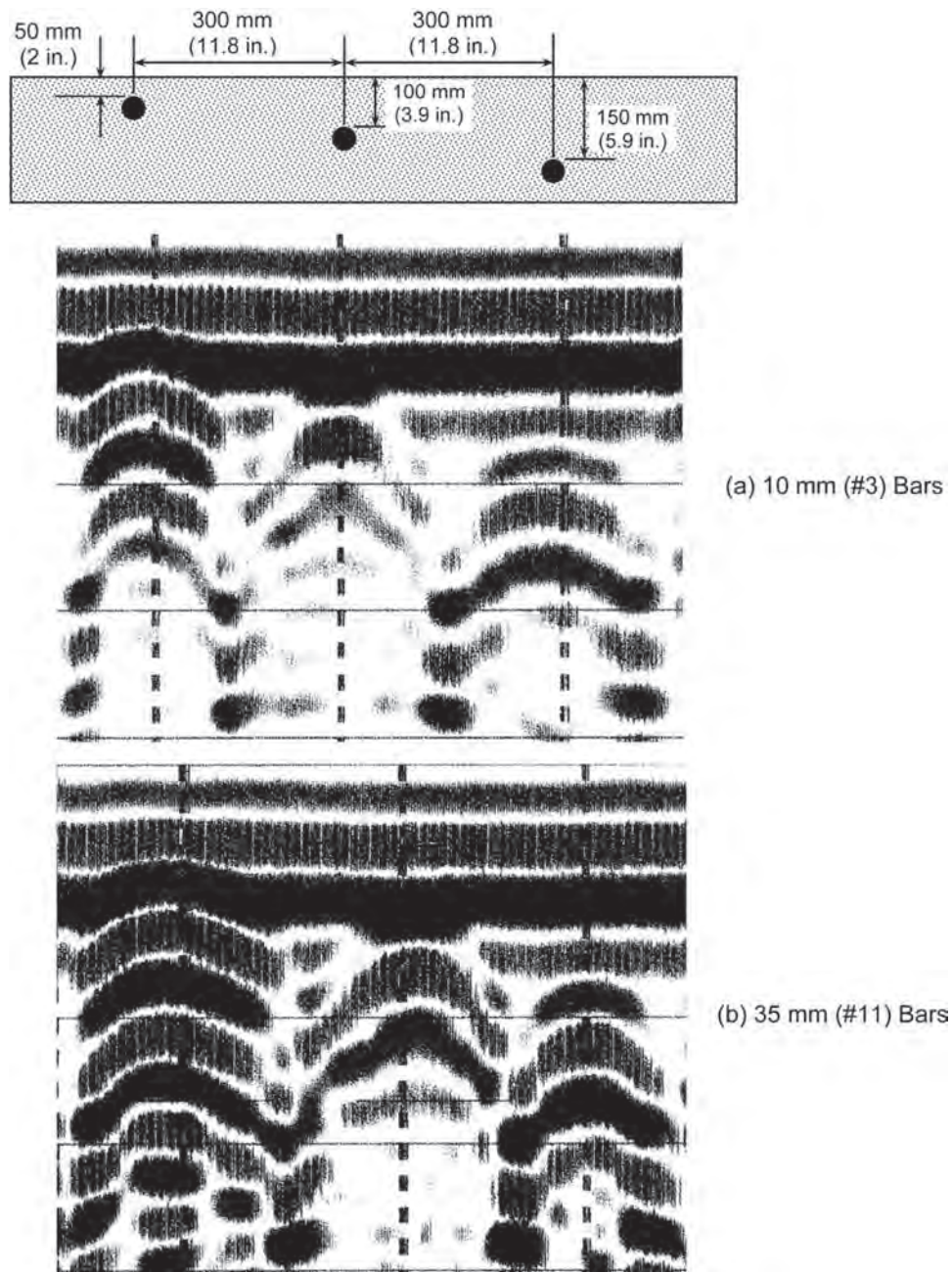
Fig. 3.8.4c—Graphic recorder displays for scans over reinforcing bars embedded at different depths in dry sand: (a) No. 3 (No. 10) bars; and (b) No. 11 (No. 36) bars.
