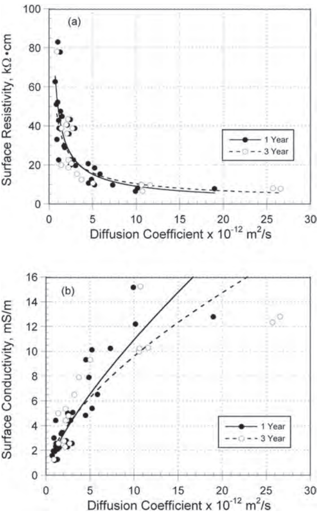
Fig. 3.5.3.5b—(a) Relationship between concrete surface resistivity at 91 days by FSTM 5-578 and apparent chloride diffusion coefficient at 1 and 3 years; and (b) same data presented as conductivity versus diffusion coefficient (adapted from Kessler et al. [2008]).
