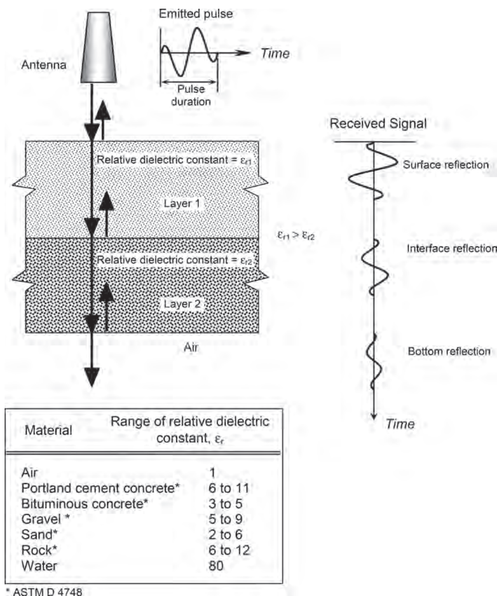
Fig. 3.8.2—Reflections of electromagnetic radiation pulse at interfaces between materials with different relative dielectric constants (adapted from Carino [1994]).
