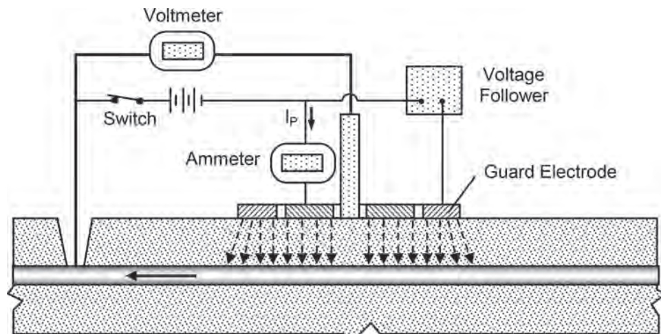
Fig. 3.5.4.2b—Linear-polarization technique using guard electrode to confine flow from counter electrode to reinforcement (adapted from Feliú et al. [1990a]).
